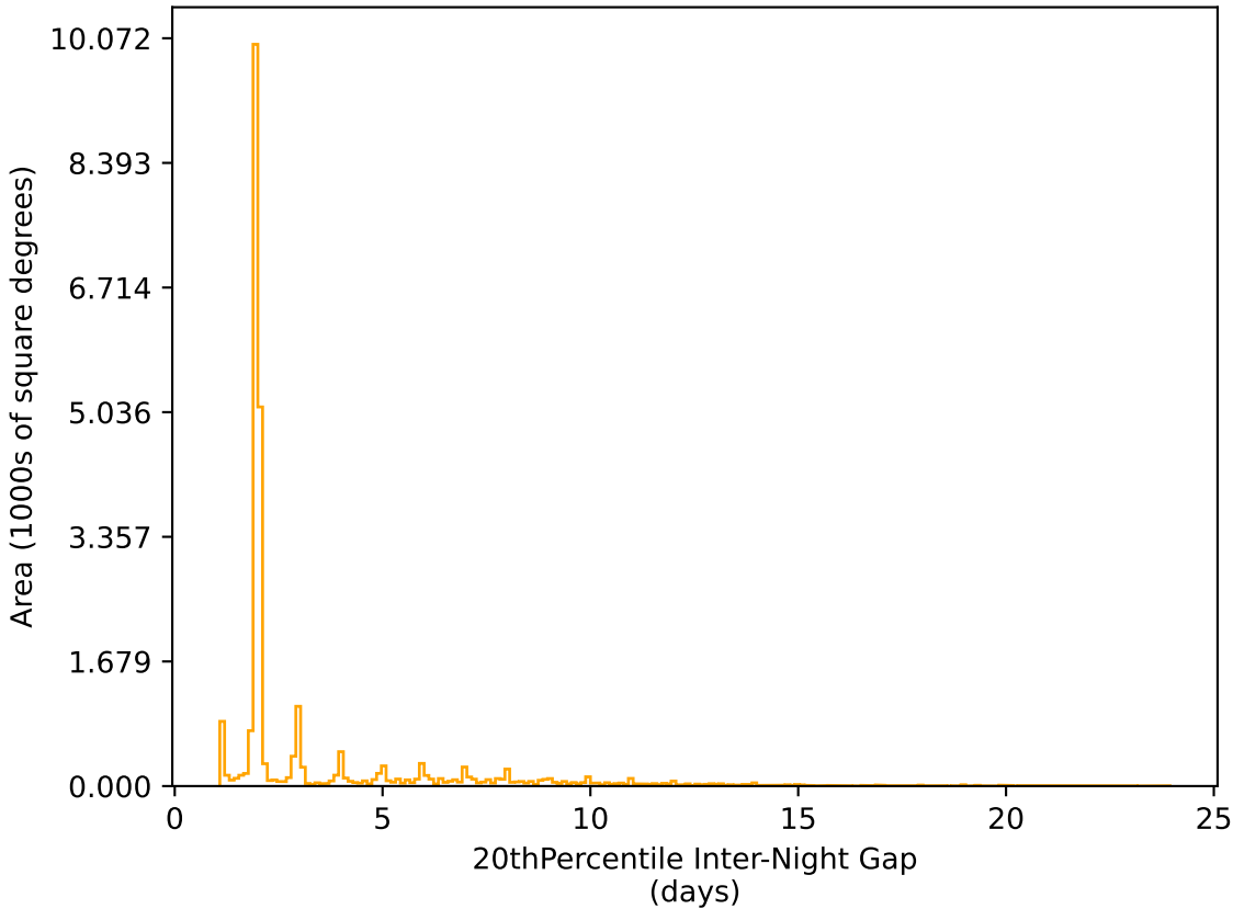
too_elab_r32_d3_giz_v3.4_10yrs All sky r band: 20thPercentile Inter-Night Gap
