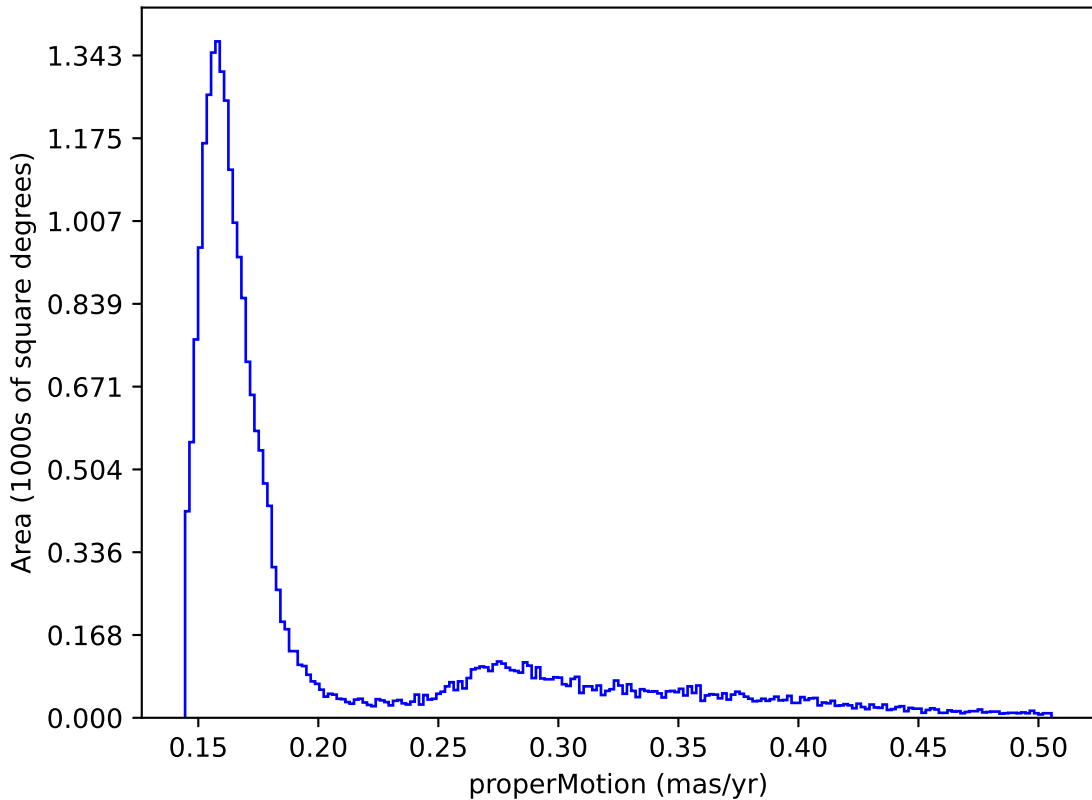
too_elab_r32_d3_giz_v3.4_10yrs : properMotion
