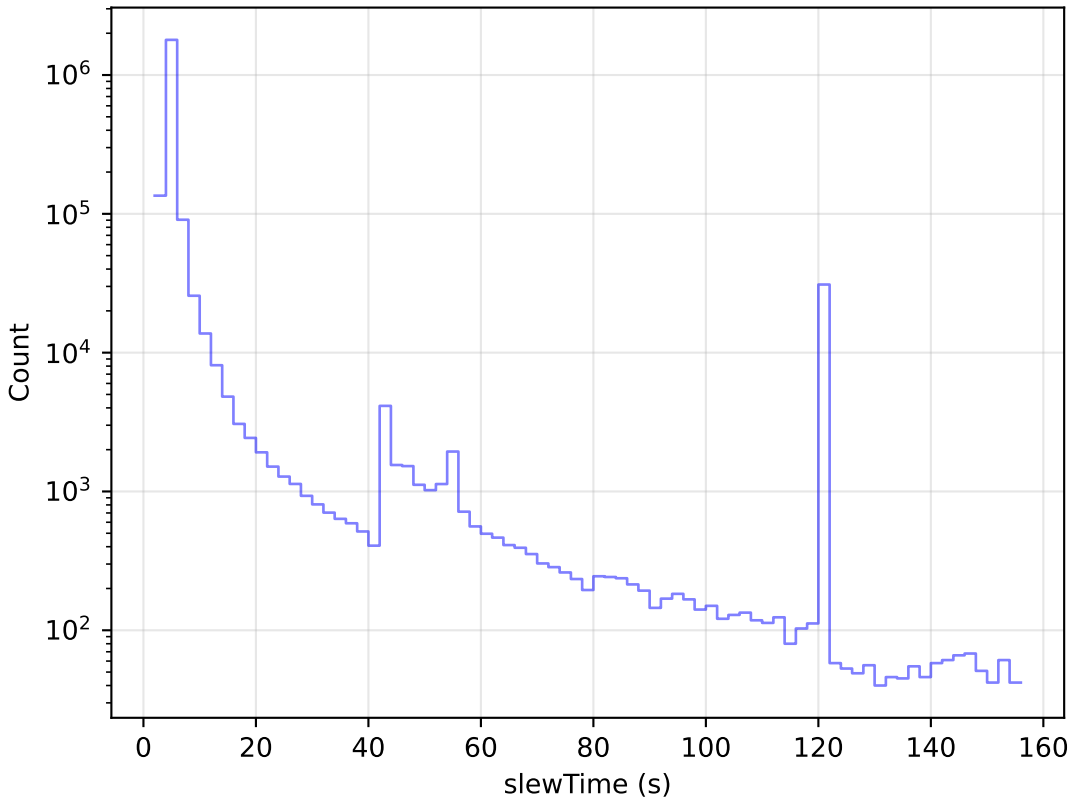
too_elab_r32_d3_giz_v3.4_10yrs All visits: Slew Time Histogram
