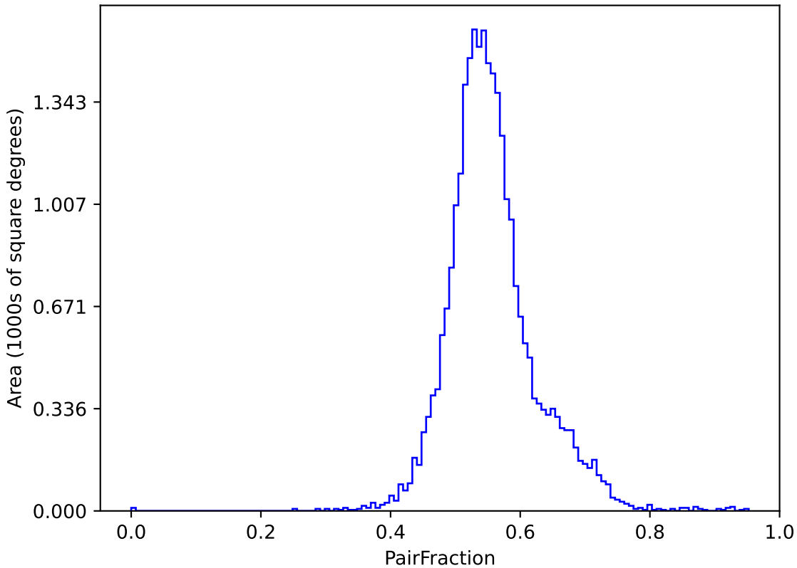
too_elab_r32_d3_giz_v3.4_10yrs (g or r or i): PairFraction
