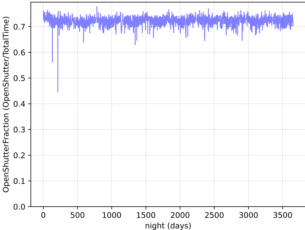
too_elab_r32_d3_giz_v3.4_10yrs : OpenShutterFraction
