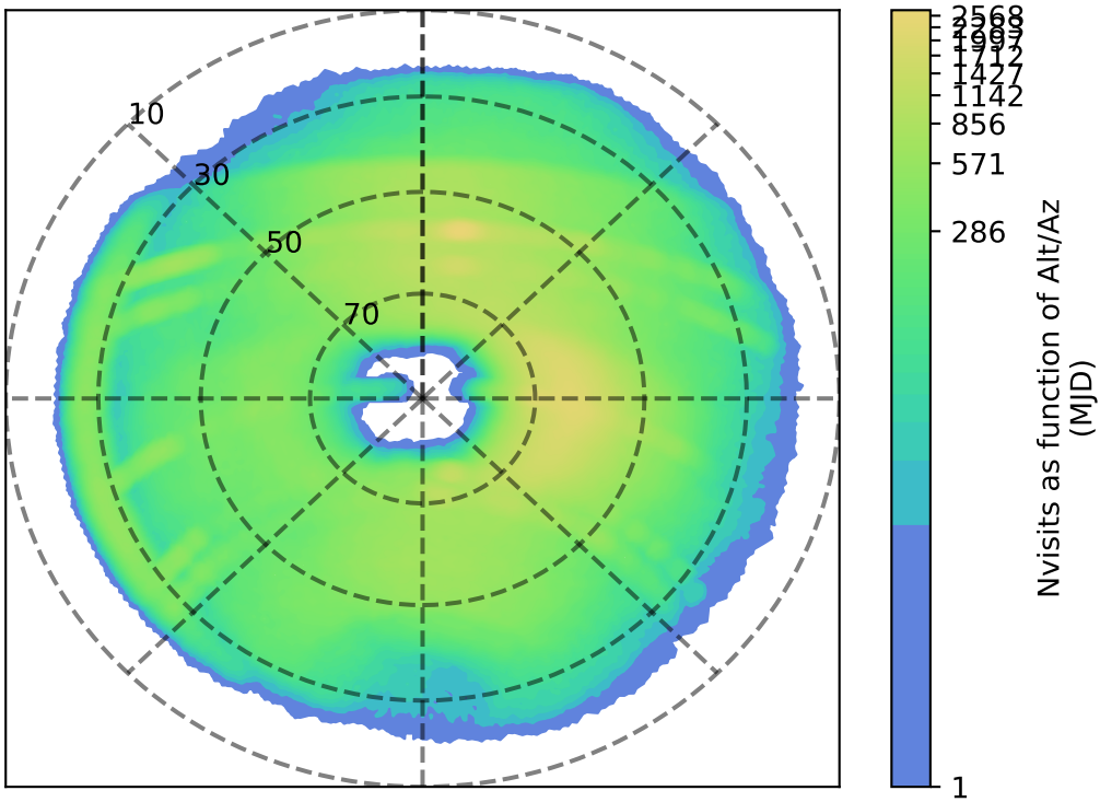
too_elab_r32_d3_giz_v3.4_10yrs r: Nvisits as function of Alt/Az
