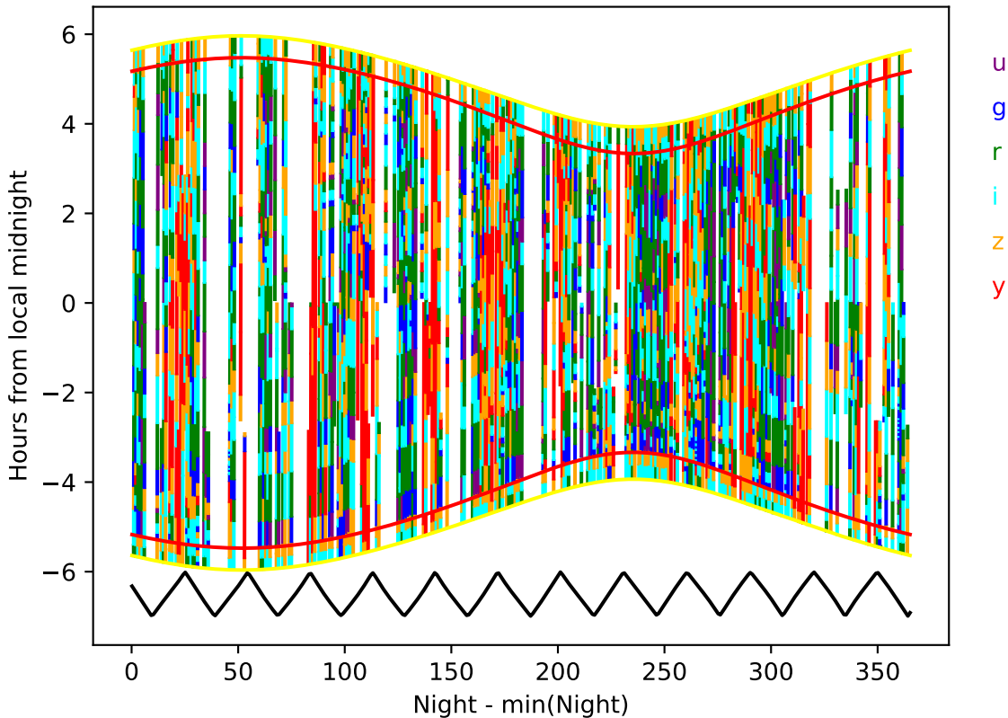
too_elab_r32_d3_giz_v3.4_10yrs year 7-8: Hourglass
