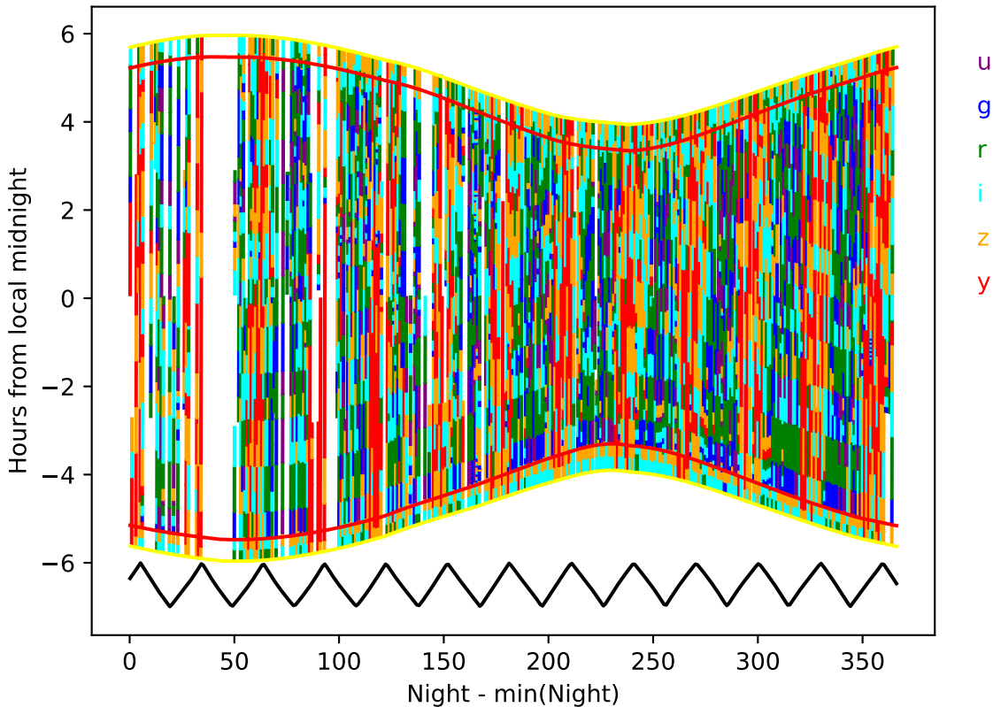
too_elab_r32_d3_giz_v3.4_10yrs year 6-7: Hourglass
