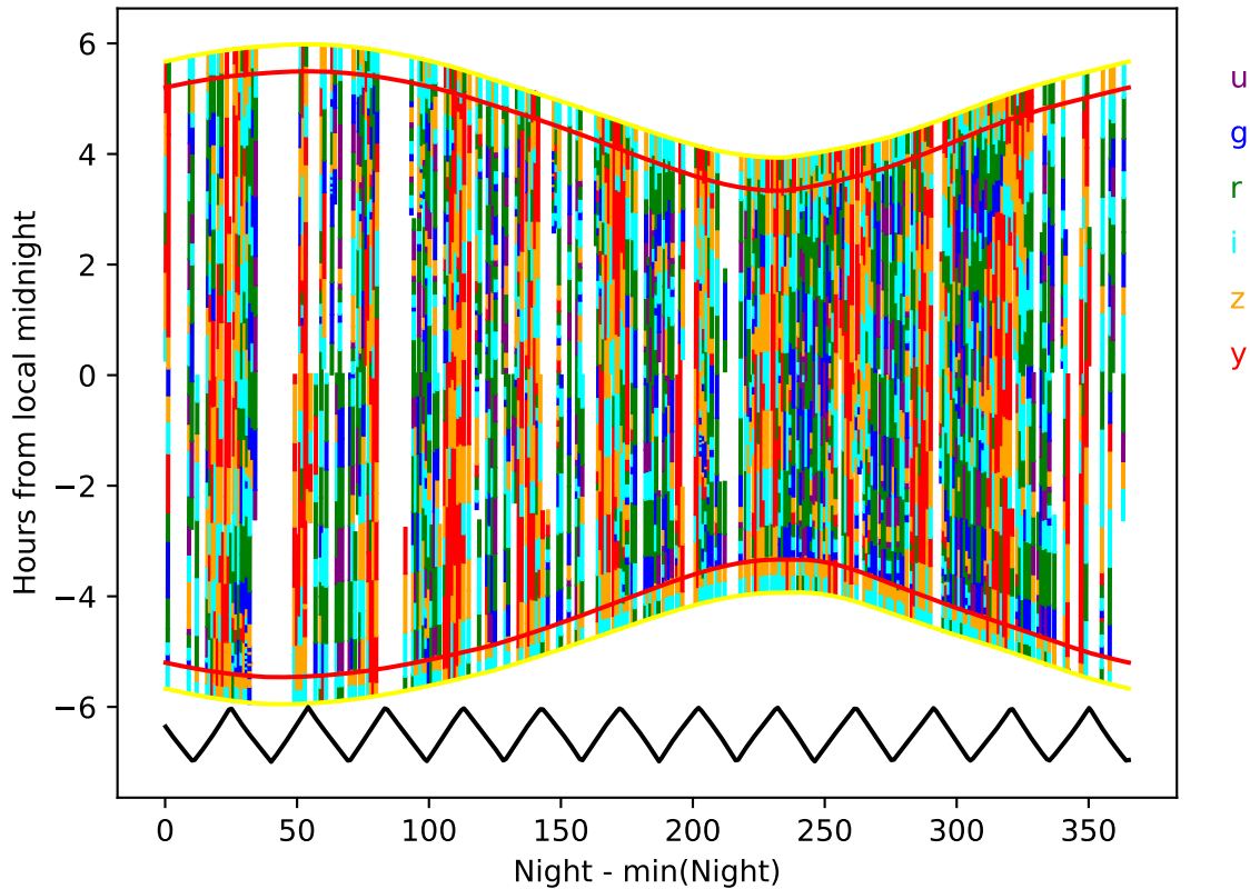
too_elab_r32_d3_giz_v3.4_10yrs year 4-5: Hourglass
