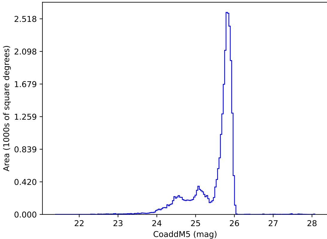
too_elab_r32_d3_giz_v3.4_10yrs z: CoaddM5
