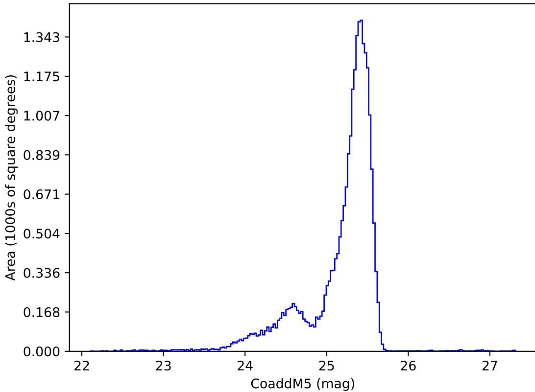
too_elab_r32_d3_giz_v3.4_10yrs u: CoaddM5
