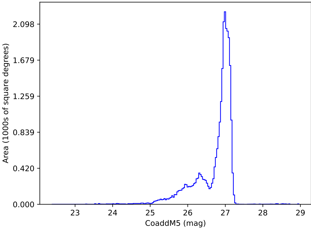
too_elab_r32_d3_giz_v3.4_10yrs r: CoaddM5
