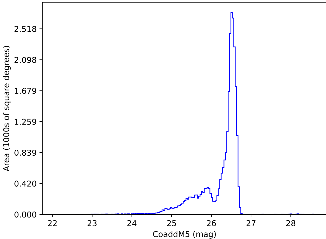
too_elab_r32_d3_giz_v3.4_10yrs i: CoaddM5
