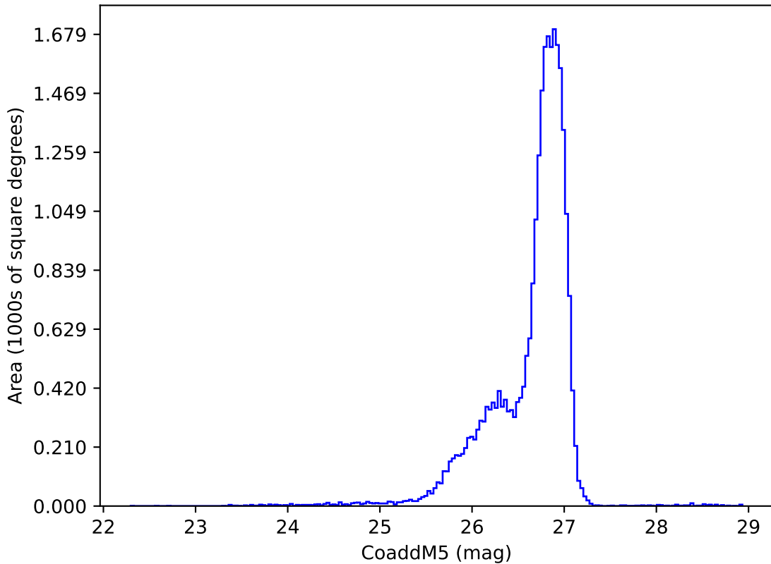
too_elab_r32_d3_giz_v3.4_10yrs g: CoaddM5
