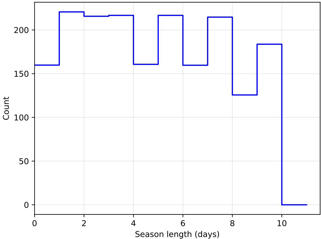
too_elab_r32_d3_giz_v3.4_10yrs DD:WFD all bands: SeasonLength
