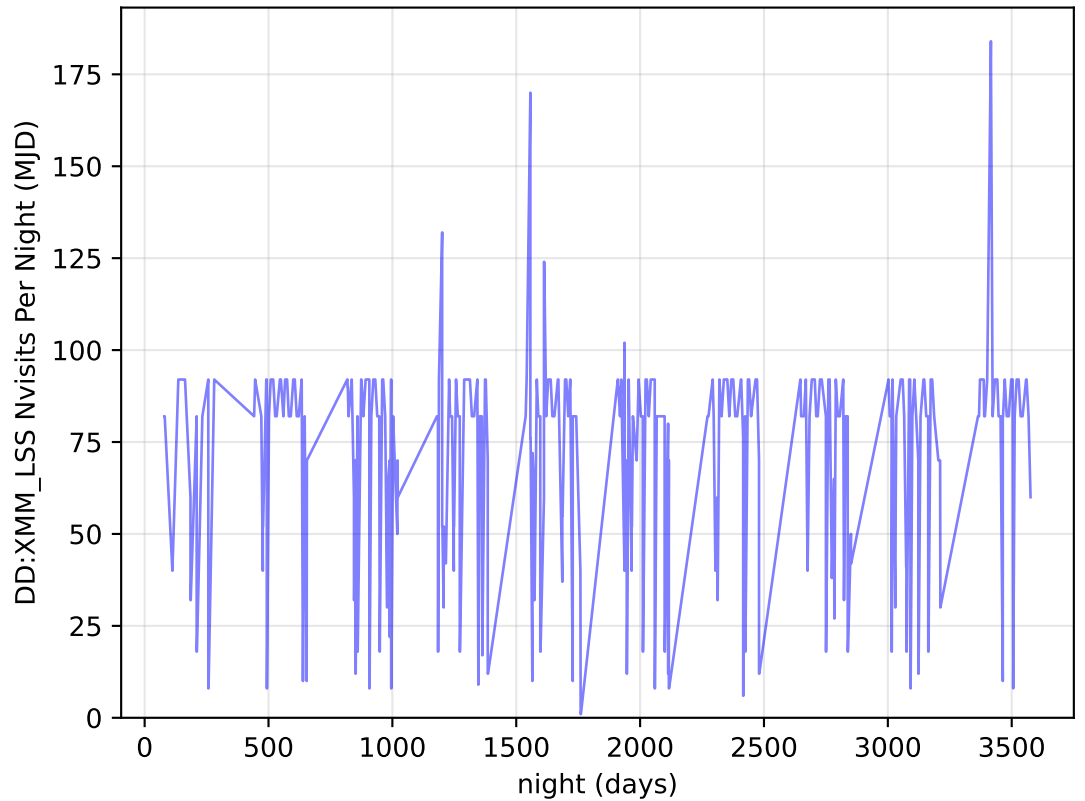
too_elab_r32_d3_giz_v3.4_10yrs all bands: DD:XMM_LSS Nvisits Per Night
