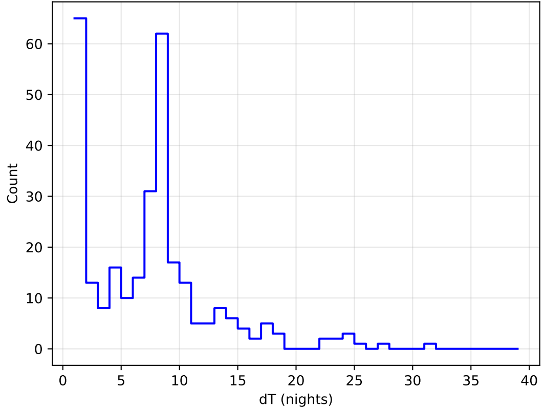
too_elab_r32_d3_giz_v3.4_10yrs all bands: DD:XMM_LSS Delta Nights Histogram
