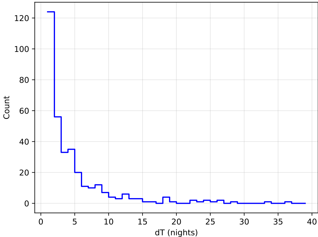
too_elab_r32_d3_giz_v3.4_10yrs all bands: DD:WFD Delta Nights Histogram
