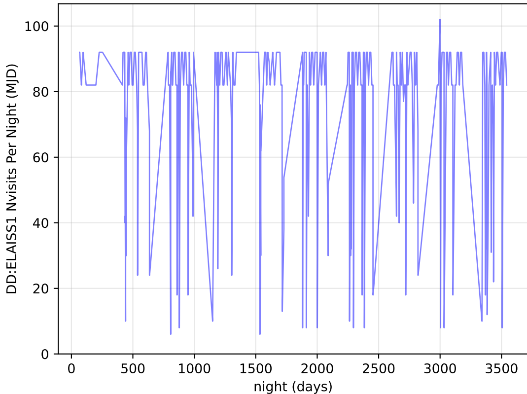
too_elab_r32_d3_giz_v3.4_10yrs all bands: DD:ELAISS1 Nvisits Per Night
