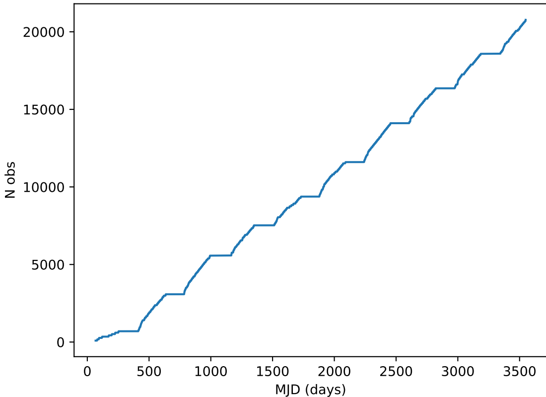
too_elab_r32_d3_giz_v3.4_10yrs all bands: DD:ELAISS1 Cumulative NVisits
