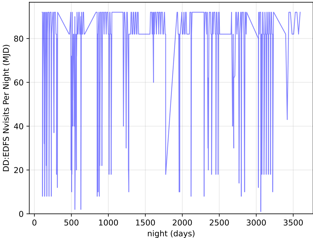
too_elab_r32_d3_giz_v3.4_10yrs all bands: DD:EDFS Nvisits Per Night
