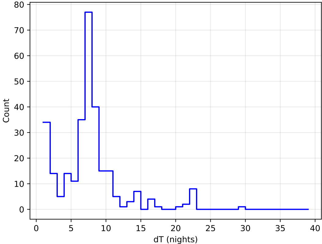
too_elab_r32_d3_giz_v3.4_10yrs all bands: DD:EDFS Delta Nights Histogram
