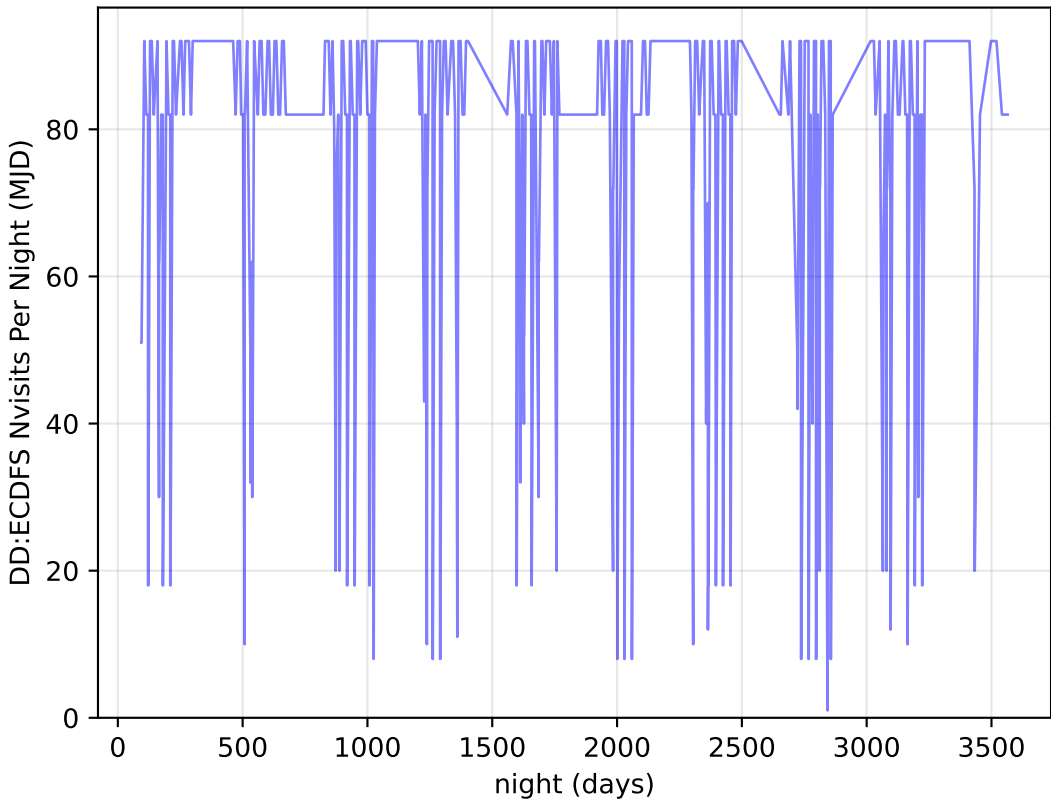
too_elab_r32_d3_giz_v3.4_10yrs all bands: DD:ECDFS Nvisits Per Night
