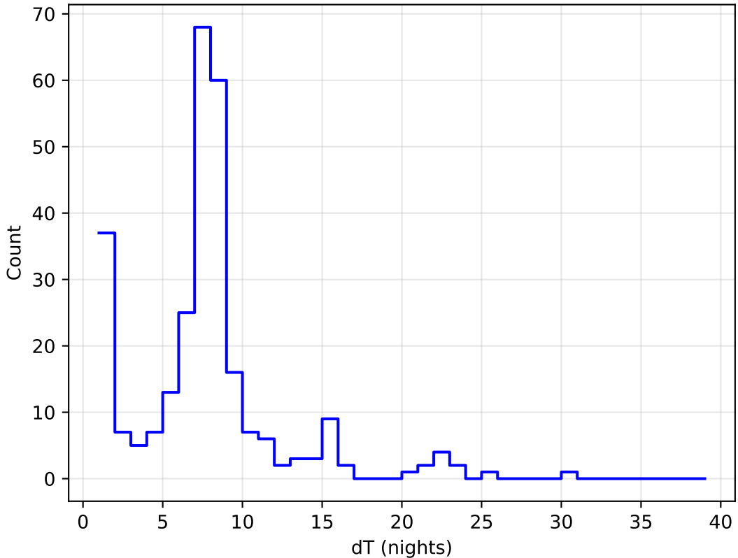
too_elab_r32_d3_giz_v3.4_10yrs all bands: DD:ECDFS Delta Nights Histogram
