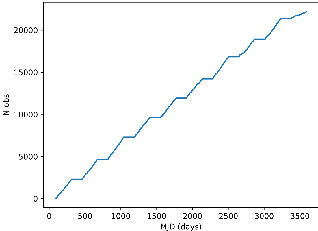
too_elab_r32_d3_giz_v3.4_10yrs all bands: DD:ECDFS Cumulative NVisits
