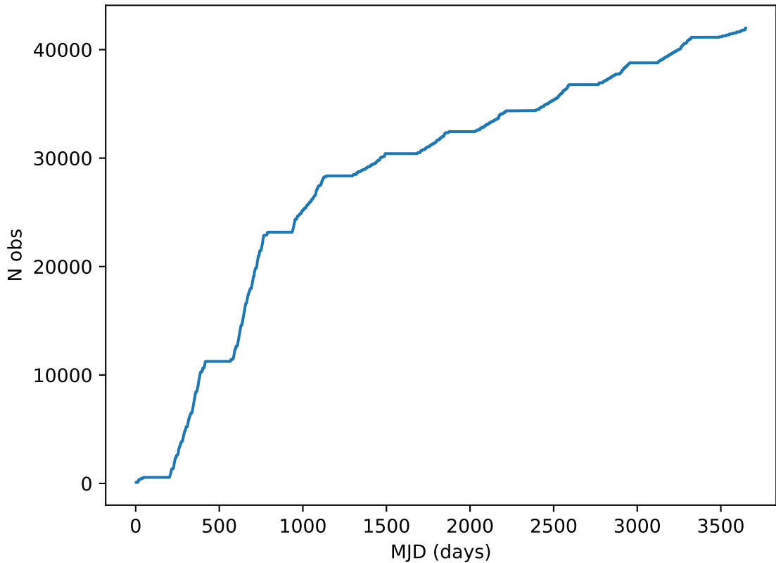
too_elab_r32_d3_giz_v3.4_10yrs all bands: DD:COSMOS Cumulative NVisits
