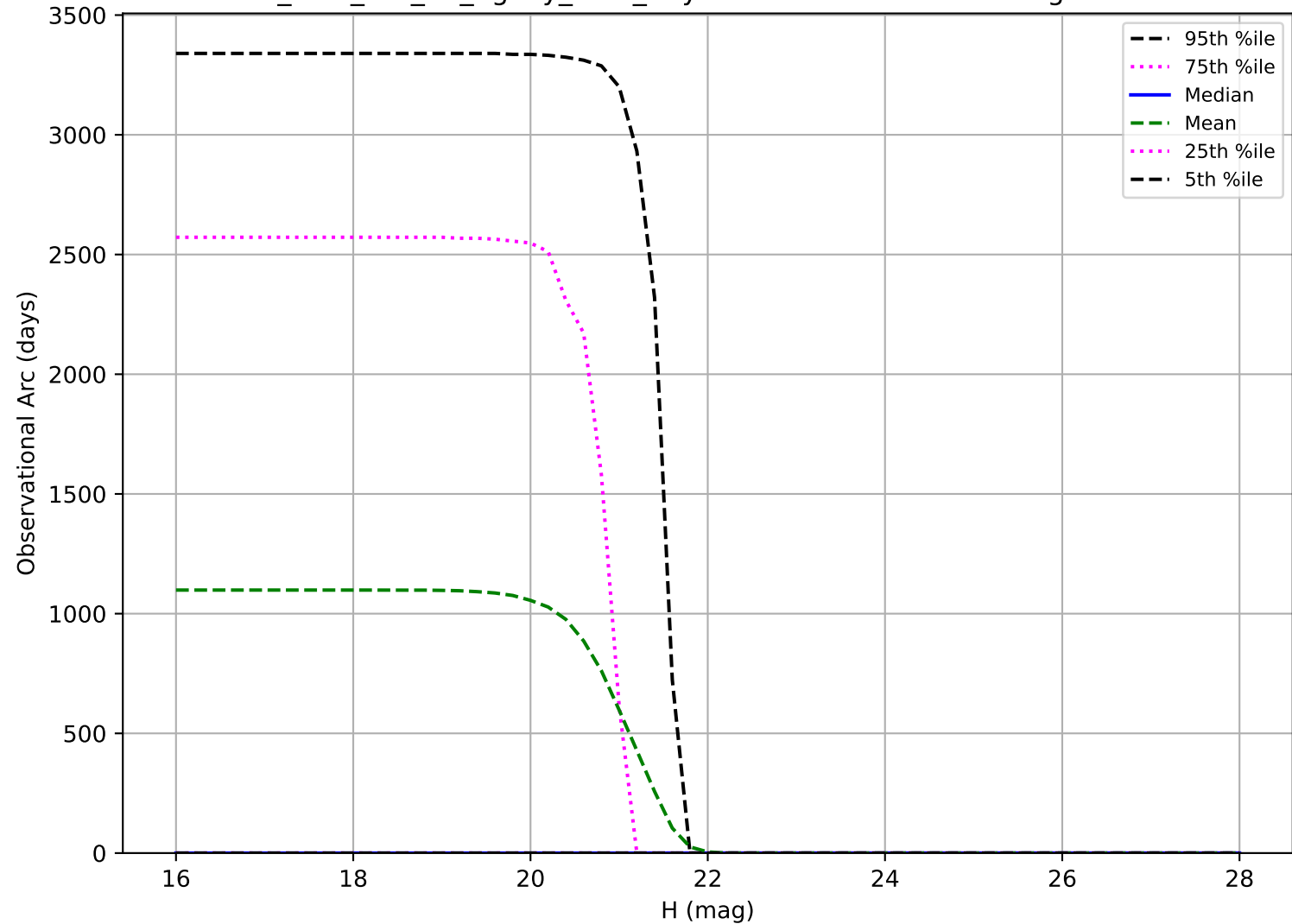
too_elab_r32_d2_ugrizy_v3.4_10yrs: Observational Arc Length Vatra
