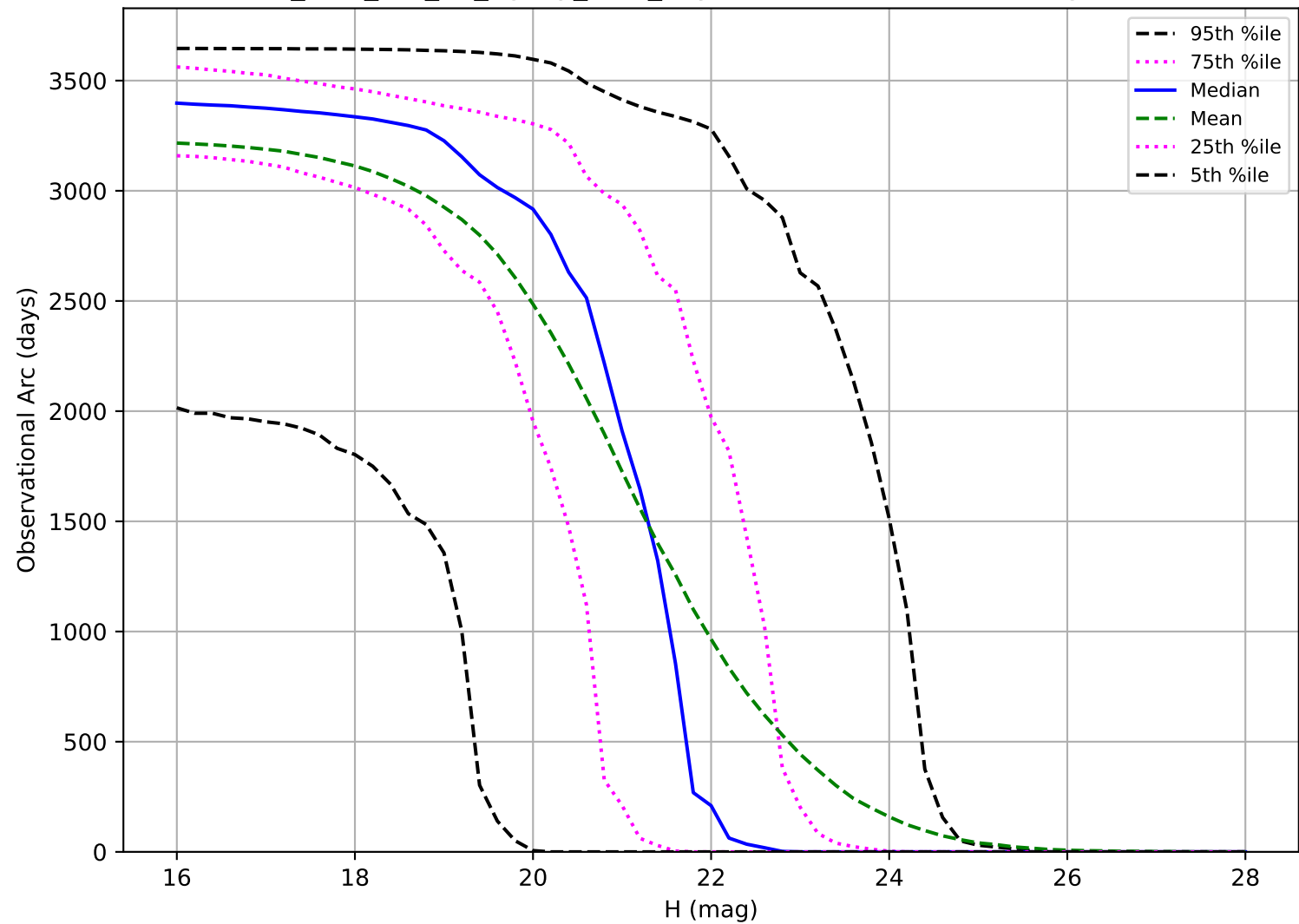
too_elab_r32_d2_ugrizy_v3.4_10yrs: Observational Arc Length PHA
