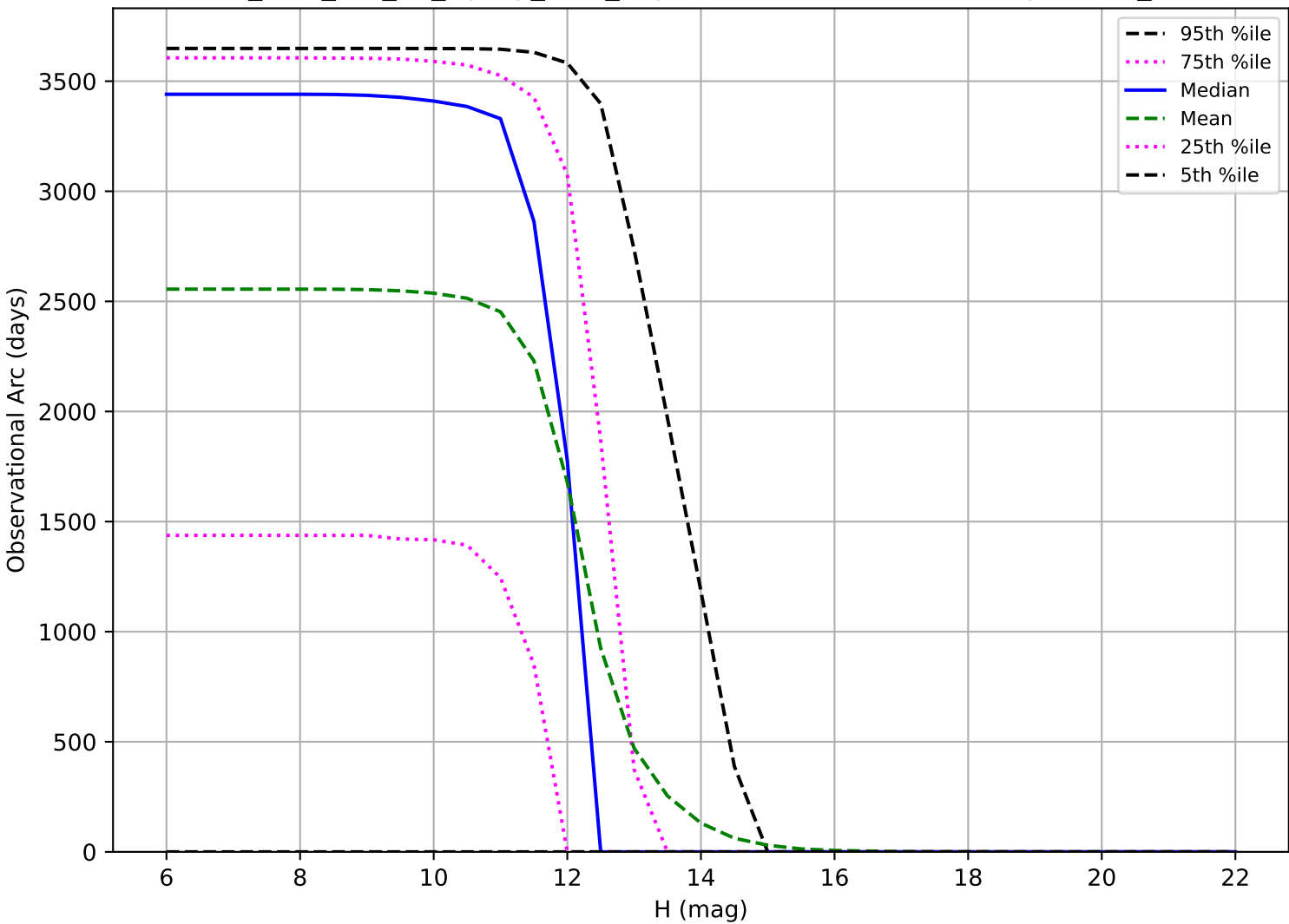
too_elab_r32_d2_ugrizy_v3.4_10yrs: Observational Arc Length OCC_r20
