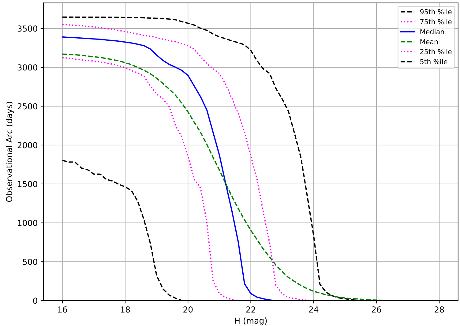
too_elab_r32_d2_ugrizy_v3.4_10yrs: Observational Arc Length NEO
