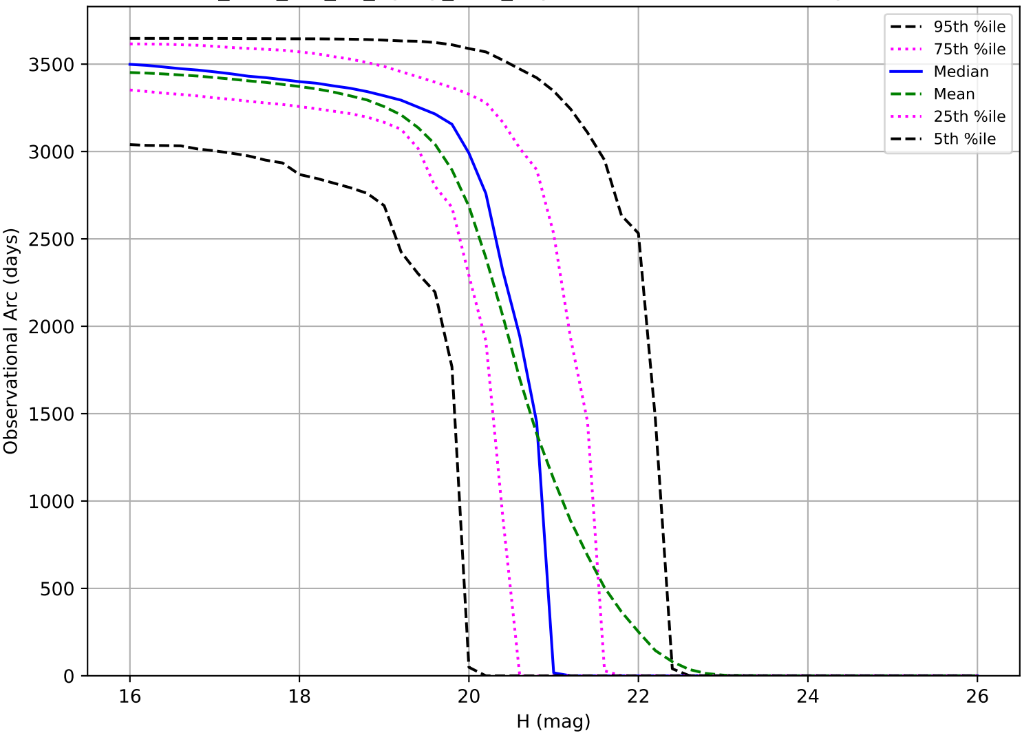
too_elab_r32_d2_ugrizy_v3.4_10yrs: Observational Arc Length MBA
