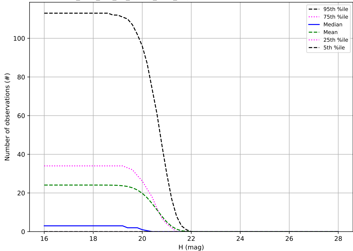
too_elab_r32_d2_ugrizy_v3.4_10yrs: Number of observations Vatira
