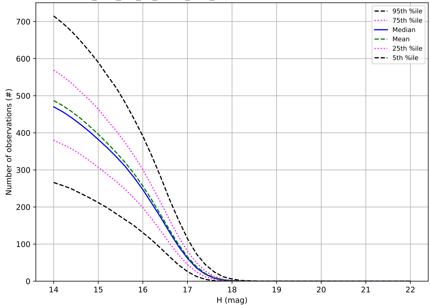
too_elab_r32_d2_ugrizy_v3.4_10yrs: Number of observations Trojan
