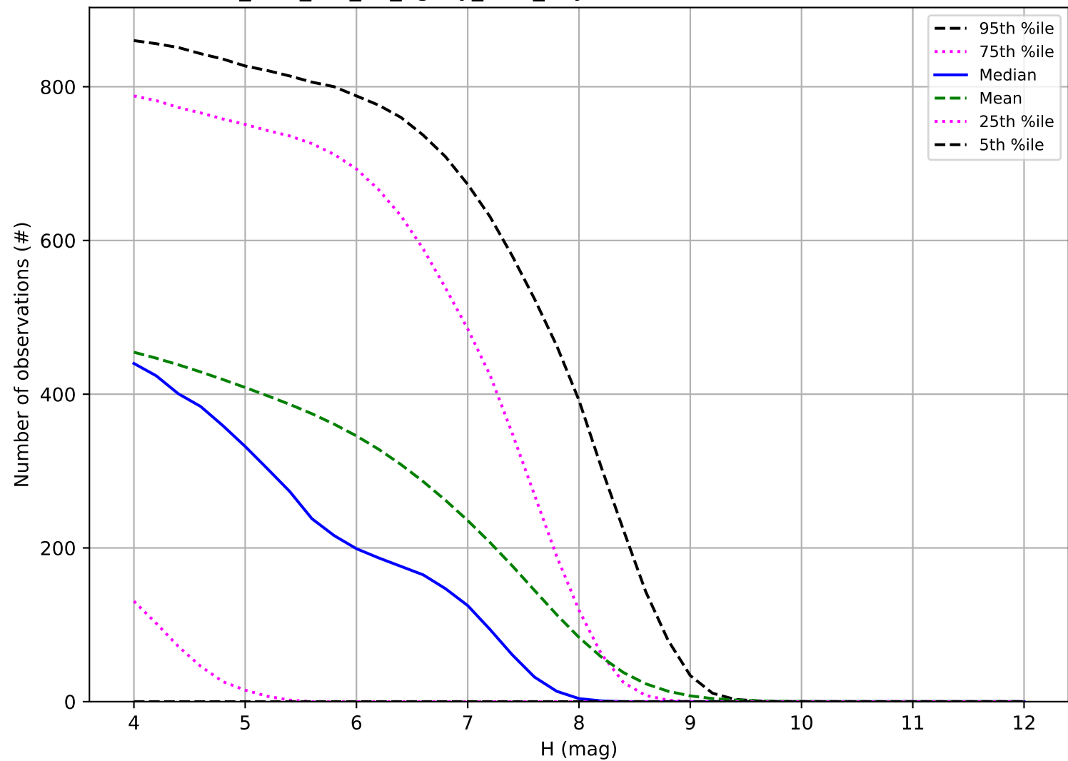
too_elab_r32_d2_ugrizy_v3.4_10yrs: Number of observations TNO
