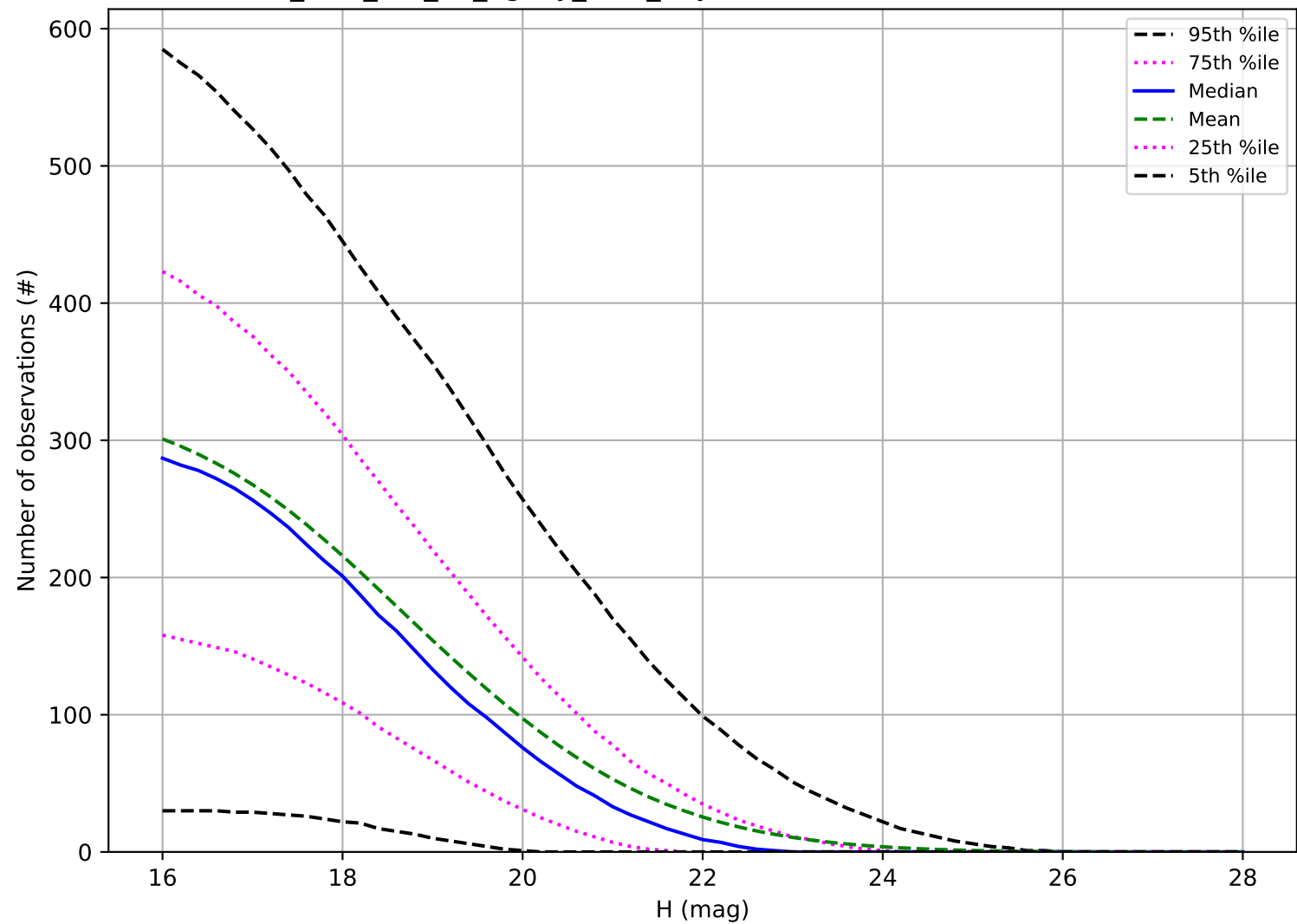
too_elab_r32_d2_ugrizy_v3.4_10yrs: Number of observations NEO
