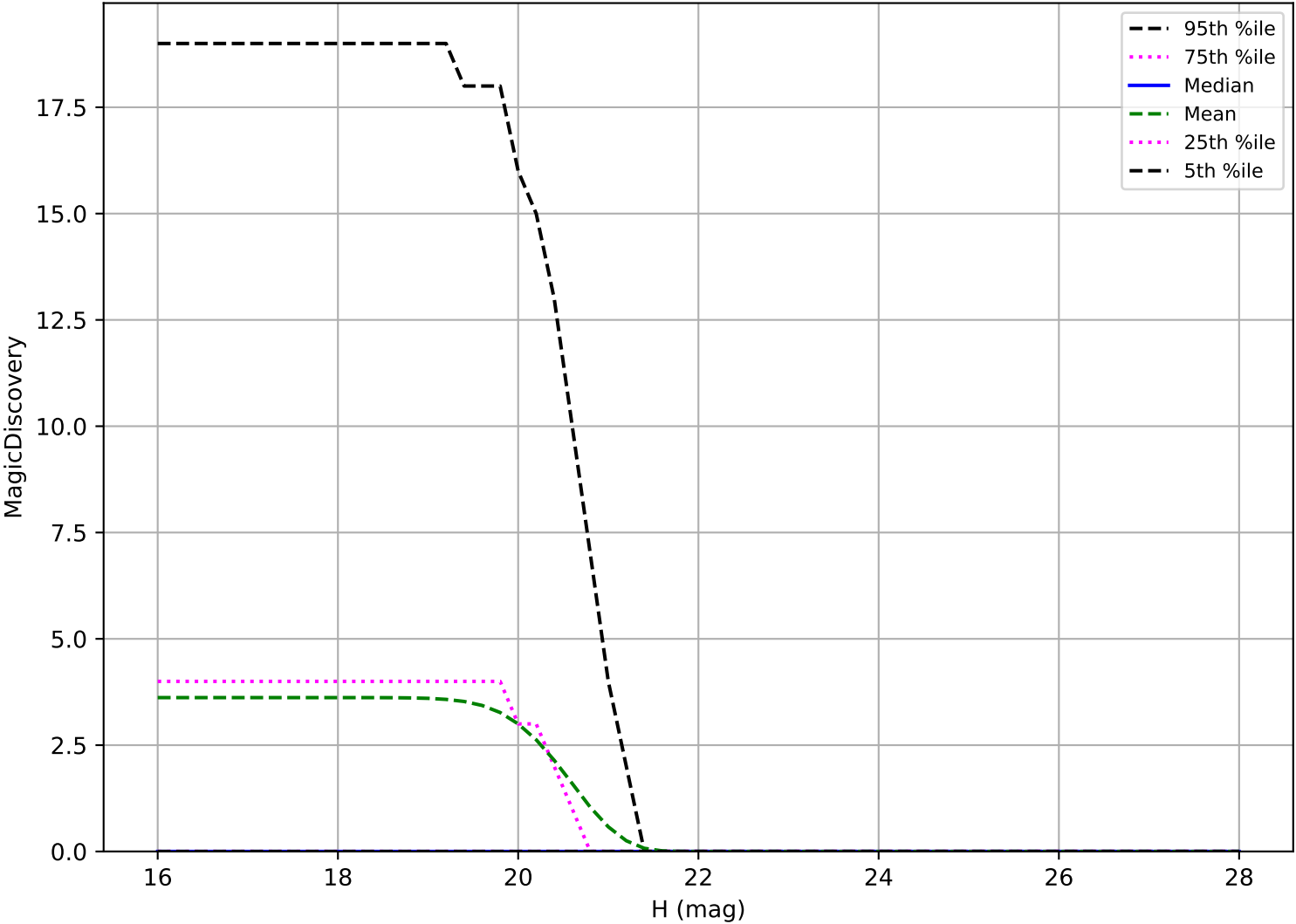
too_elab_r32_d2_ugrizy_v3.4_10yrs: Vatira 6 detections in 60 nights detection loss
