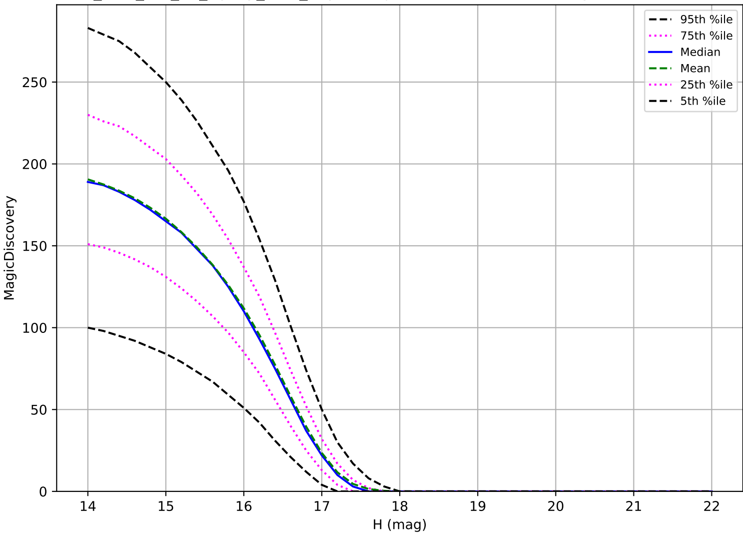
too_elab_r32_d2_ugrizy_v3.4_10yrs: Trojan 6 detections in 60 nights detection loss
