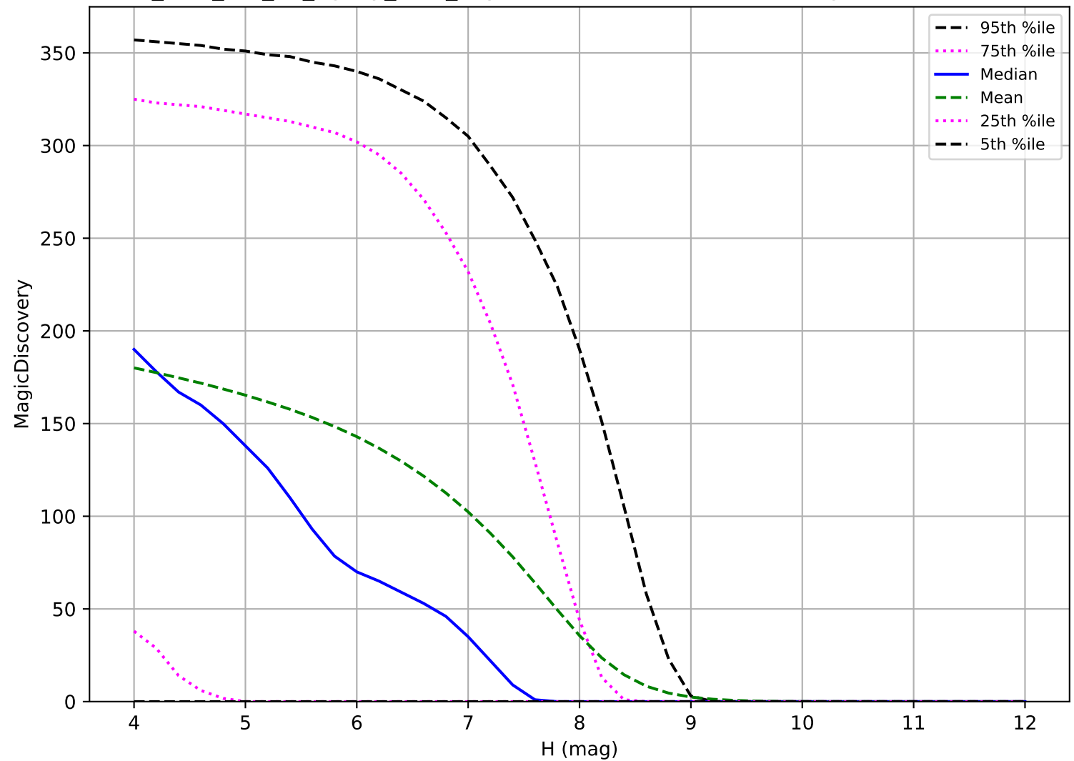
too_elab_r32_d2_ugrizy_v3.4_10yrs: TNO 6 detections in 60 nights detection loss
