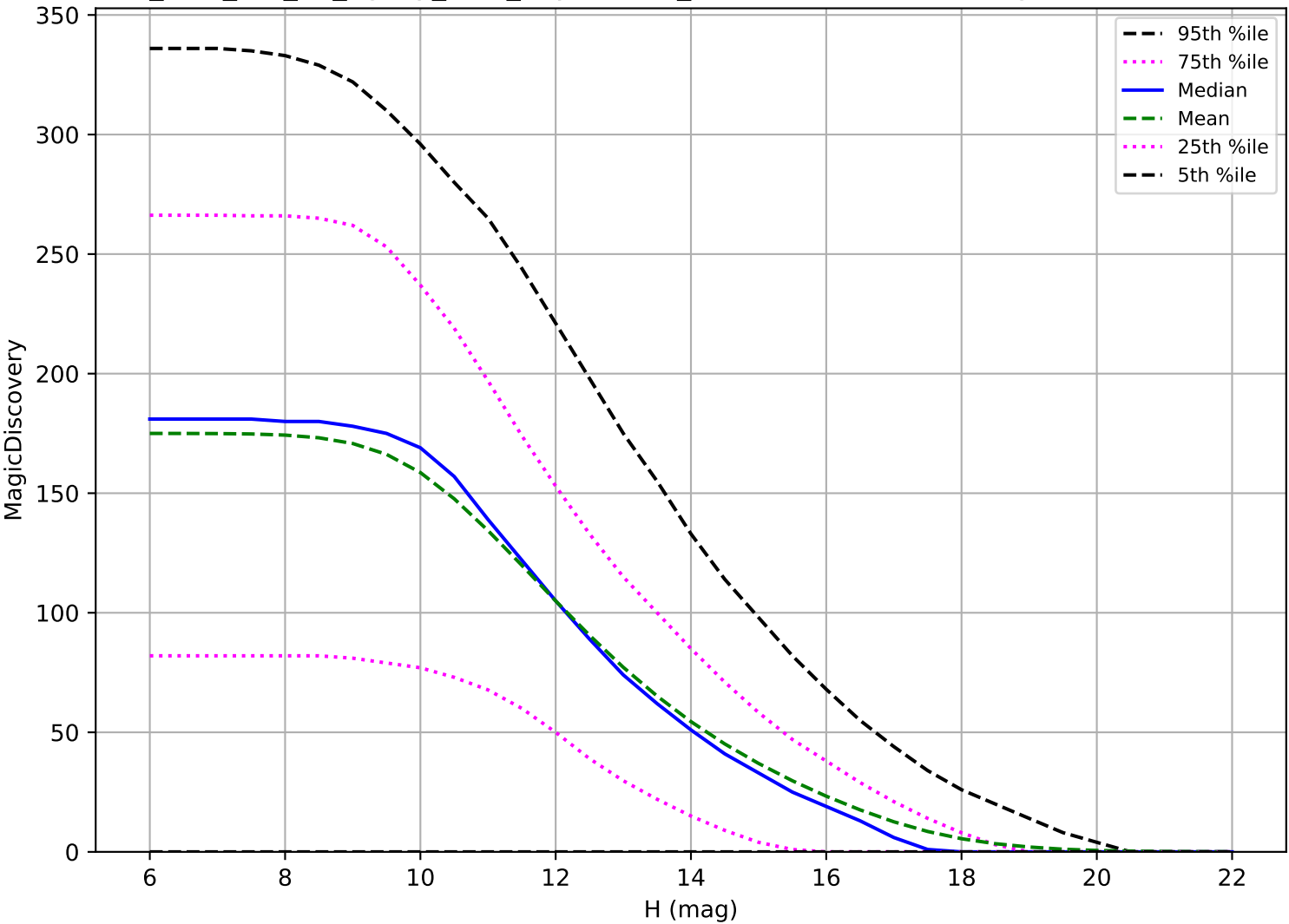
too_elab_r32_d2_ugrizy_v3.4_10yrs: OCC_r5 6 detections in 60 nights detection loss
