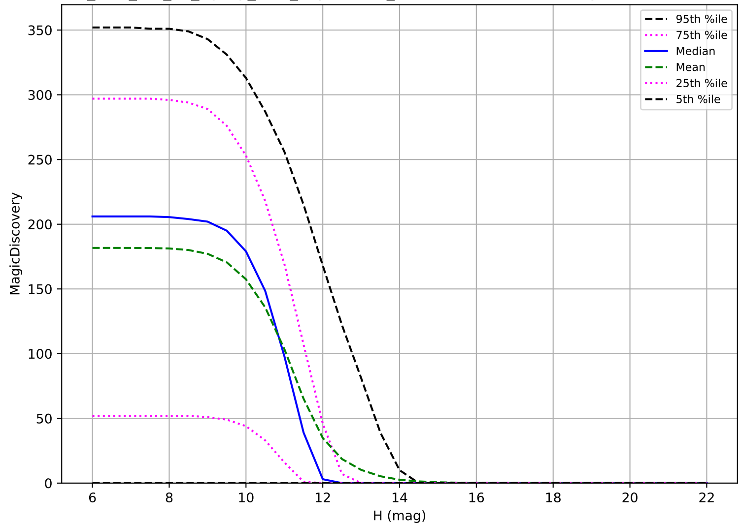
too_elab_r32_d2_ugrizy_v3.4_10yrs: OCC_r20 6 detections in 60 nights detection loss
