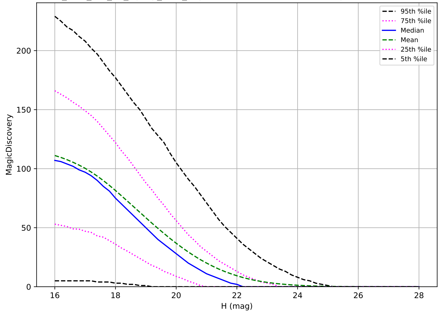
too_elab_r32_d2_ugrizy_v3.4_10yrs: NEO 6 detections in 60 nights detection loss
