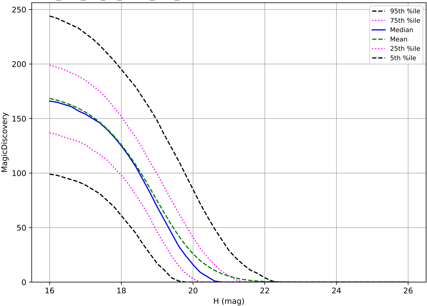
too_elab_r32_d2_ugrizy_v3.4_10yrs: MBA 6 detections in 60 nights detection loss
