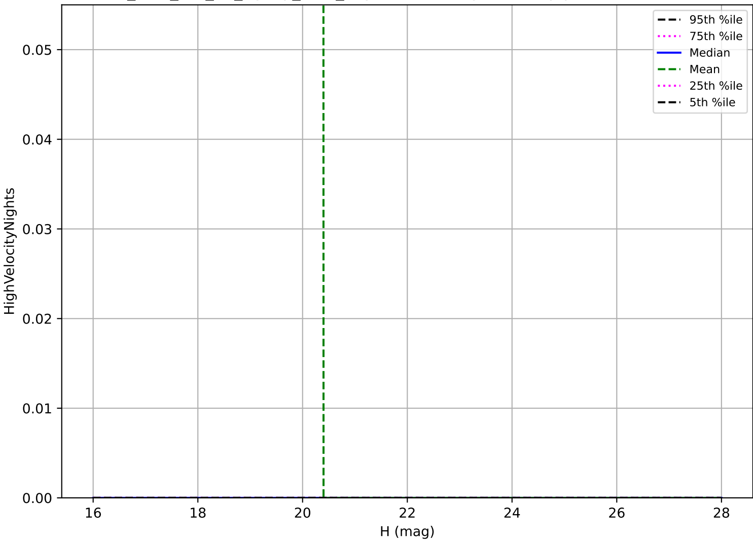
too_elab_r32_d2_ugrizy_v3.4_10yrs: Vatira High velocity pair detection loss
