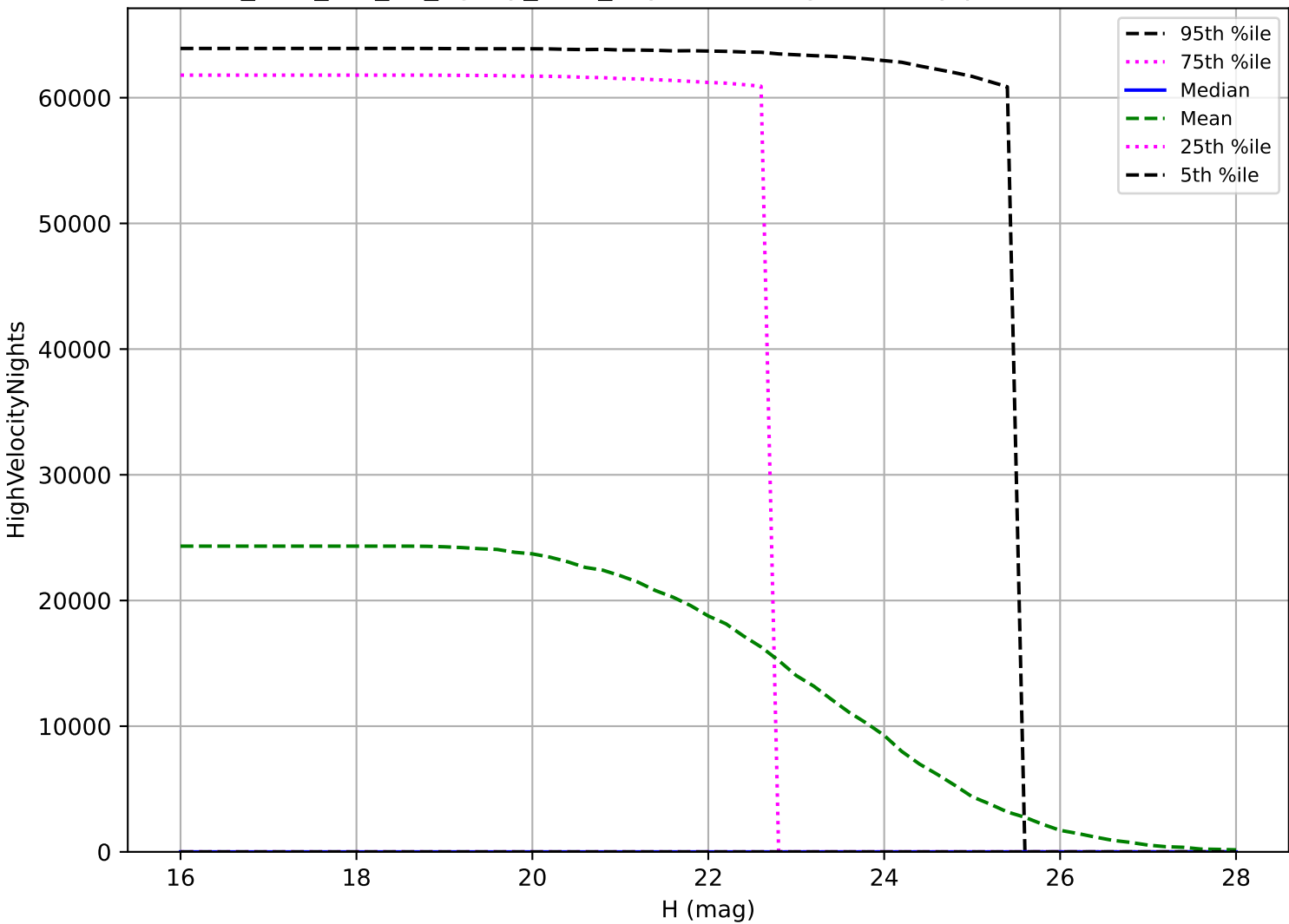
too_elab_r32_d2_ugrizy_v3.4_10yrs: PHA High velocity pair detection loss
