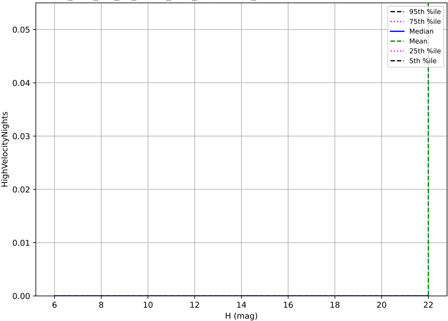
too_elab_r32_d2_ugrizy_v3.4_10yrs: OCC_r20 High velocity pair detection loss
