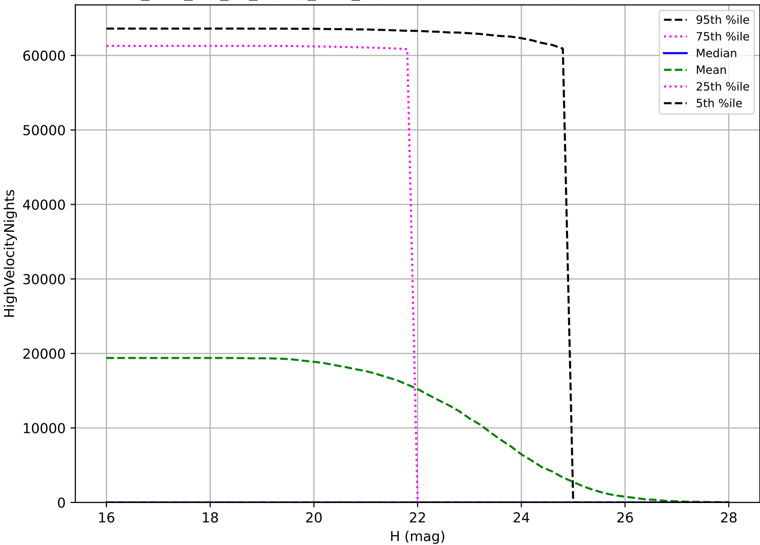
too_elab_r32_d2_ugrizy_v3.4_10yrs: NEO High velocity pair detection loss
