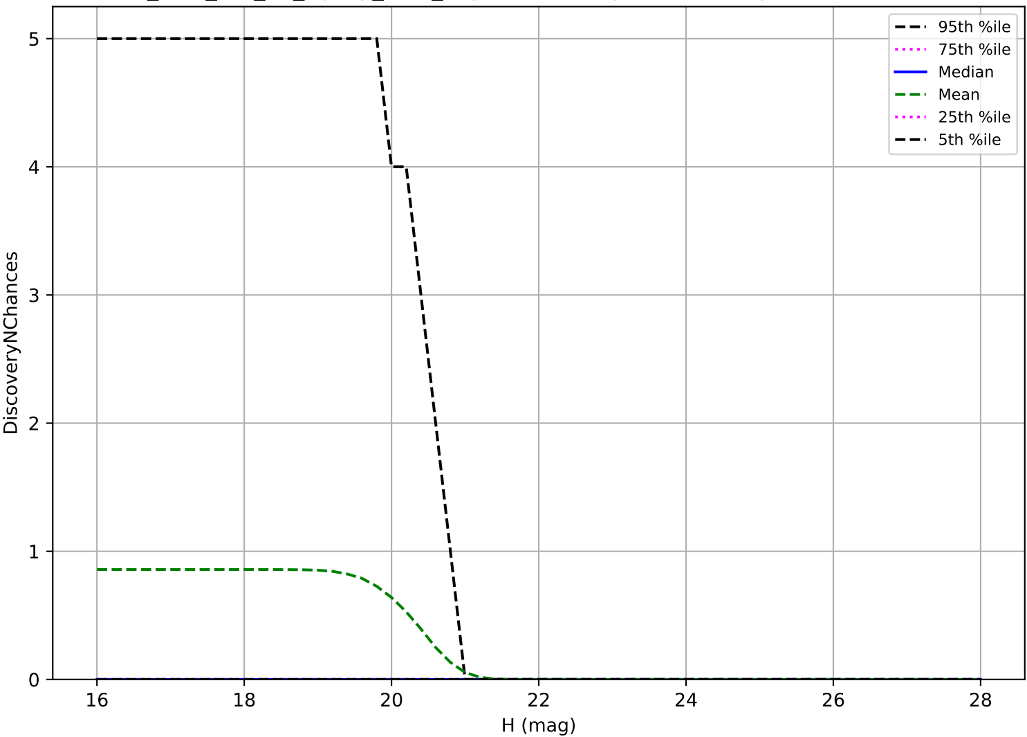
too_elab_r32_d2_ugrizy_v3.4_10yrs: Vatira 3 pairs in 15 nights detection loss
