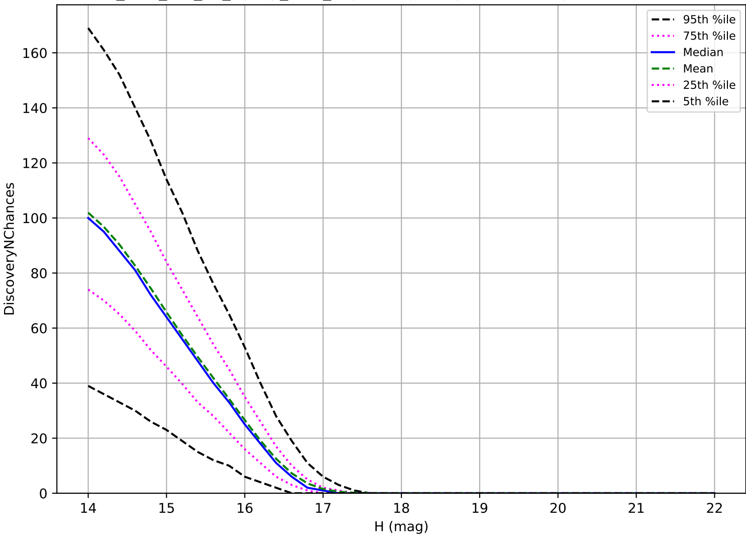
too_elab_r32_d2_ugrizy_v3.4_10yrs: Trojan 3 pairs in 15 nights detection loss
