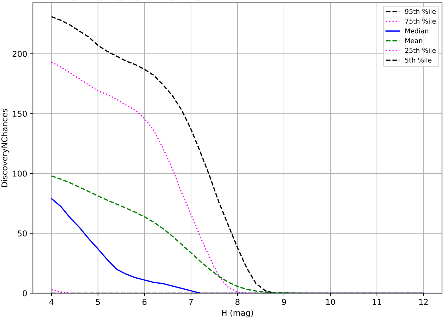
too_elab_r32_d2_ugrizy_v3.4_10yrs: TNO 3 pairs in 15 nights detection loss
