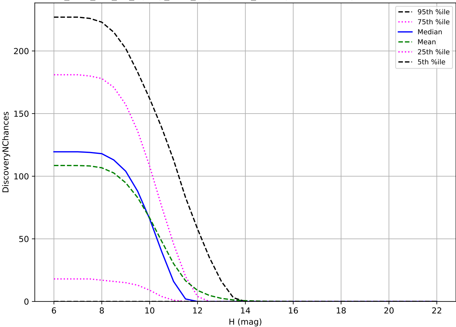
too_elab_r32_d2_ugrizy_v3.4_10yrs: OCC_r20 3 pairs in 15 nights detection loss
